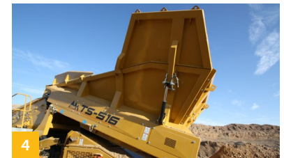
4 The heavy-duty, direct-feed system includes a rubber belt feeder and an optional HARDOX® apron feeder for increased longevity in rigorous applications.
