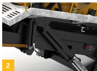
2 Hydraulic Screenbox linkage system, allows greater accessibility for screen change and enables optimum screen coverage at varying screenbox angles.
