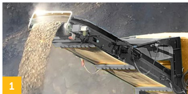
1 Large gap between crusher discharge and the main conveyor feedboot prevents bottlenecks.
